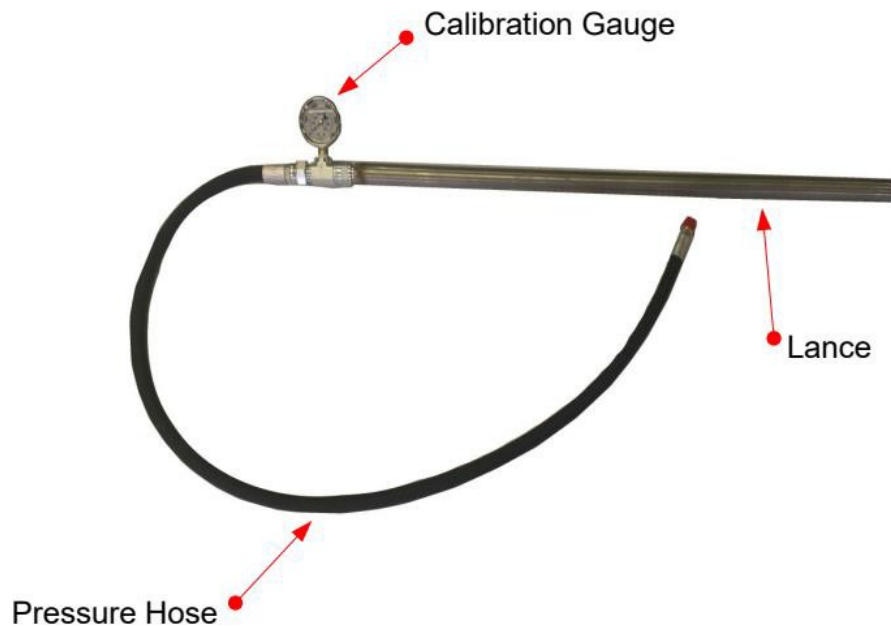
Figure 5.2 – Lance Pressure Calibration
