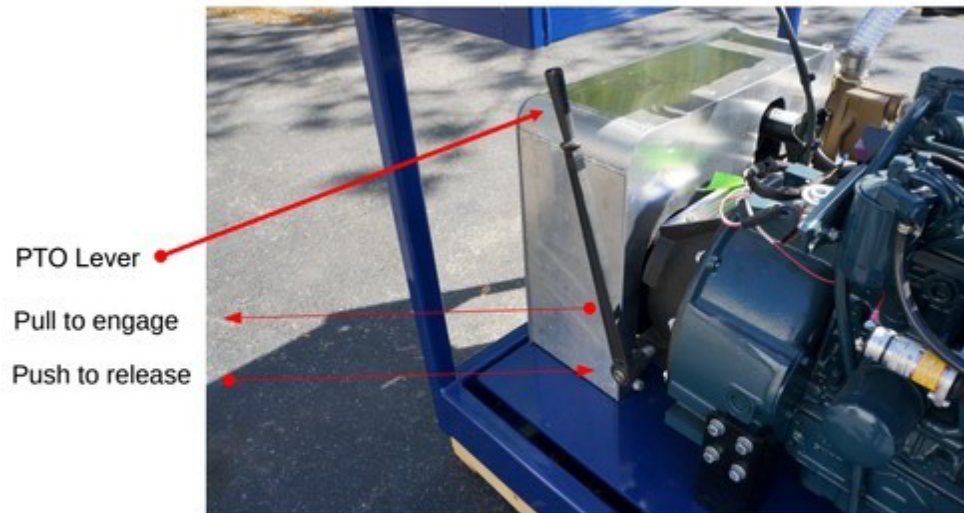
PTO Lever To Engage and Disengage Clutch
