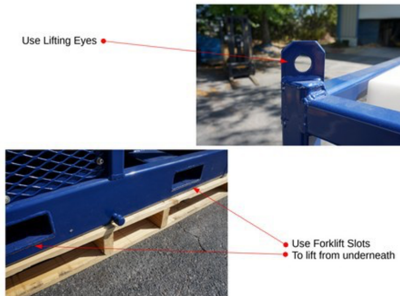
Figure 4.1 – Lifting Guidelines
