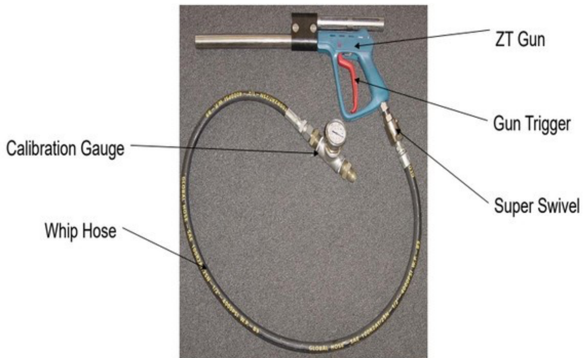
Figure 5.3 – Gun Pressure Calibration
