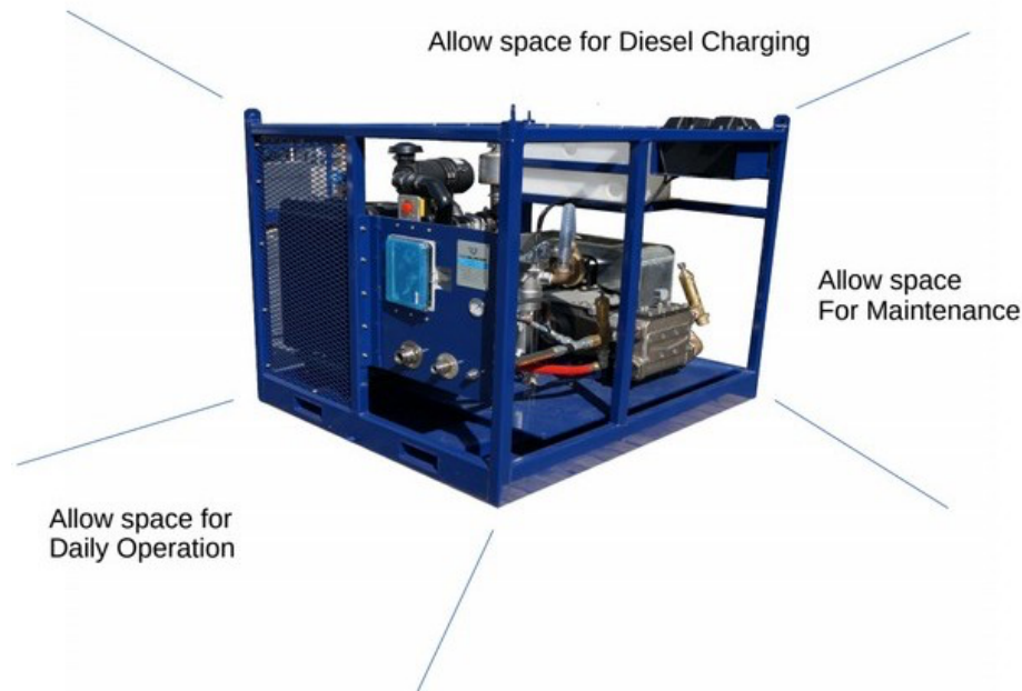
Figure 4.2 – Installation Guidelines
