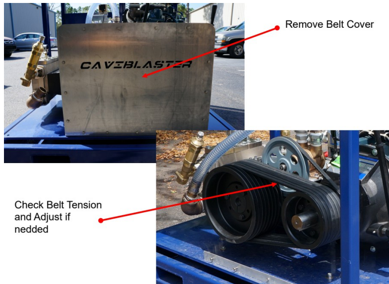
Figure 6.2 – Belt Inspection / Tension
