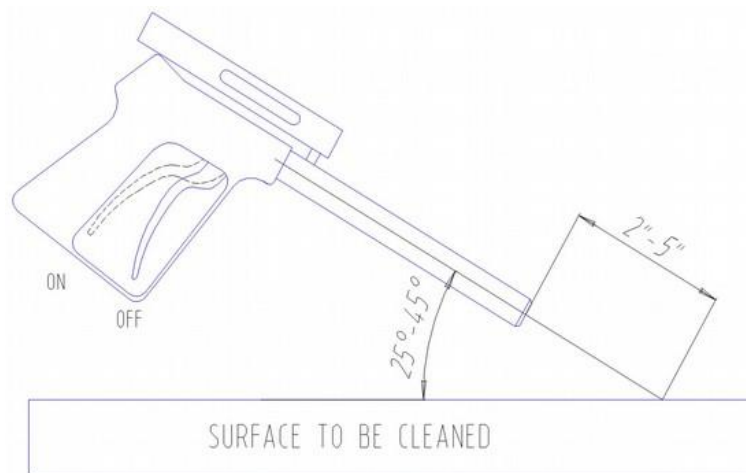
Figure 18 – Gun Position for Best Results
